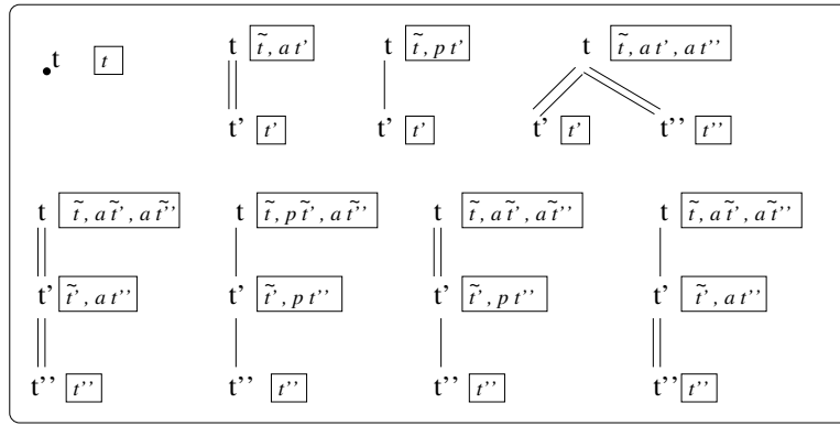
Fig. 6 Information Propagation Examples
