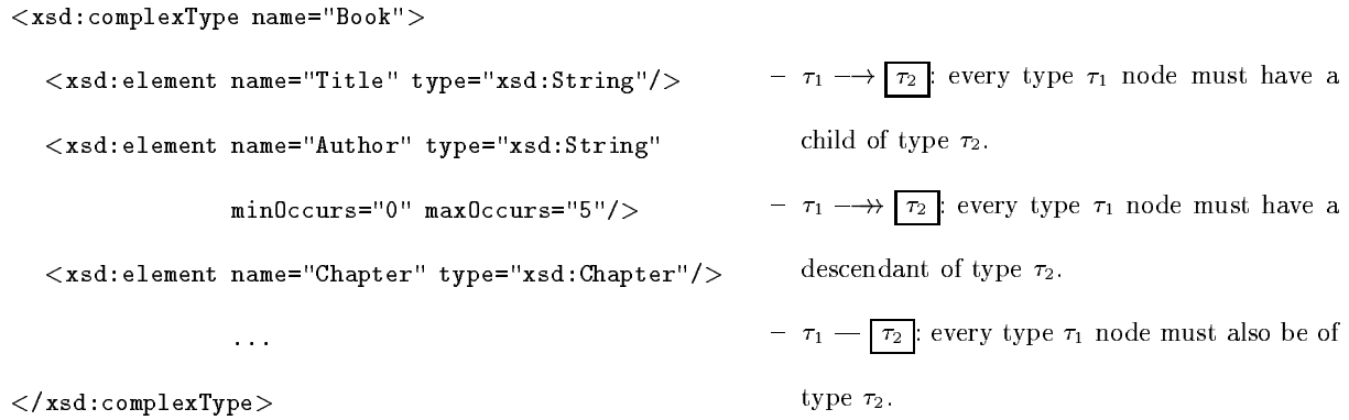
(a) Example XML Schema Specification
