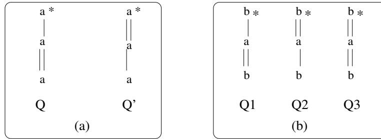
Fig. 3 Counterexamples to the necessity of containment mappings on databases over a small alphabet.
