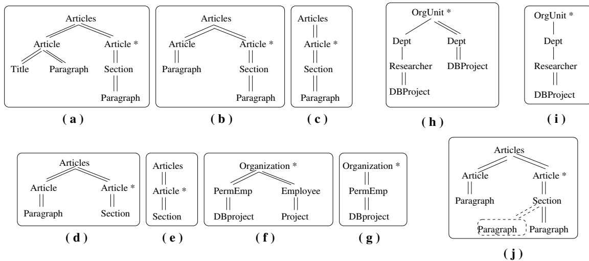
Fig. 2 Examples of Tree Pattern Queries
