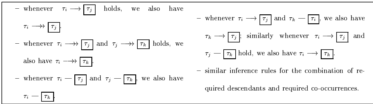
Fig. 5 Inference Rules
