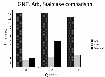
Figure 1: Staircase Join, Arb and GNF.
