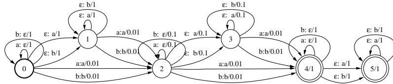
Fig. 1. Gappy bigram rational kernel with decay factor \lambda = .1 . Bold face circles represent initial states and double circles indicate final states.
