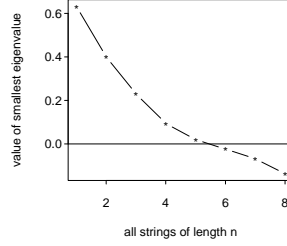
Fig. 3. Value of the smallest eigenvalue of the matrix M_n = (\exp(-d_e(x_i, x_j)))_{1 \leq i, j, \leq 2^n} as a function of n .
