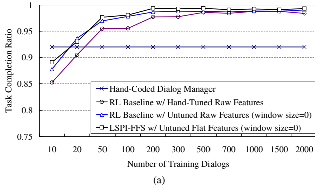
Figure 1: Average task completion ratios of policies learned by various algorithms. Average total rewards and average interaction lengths had qualitatively similar curves. See text for details.
