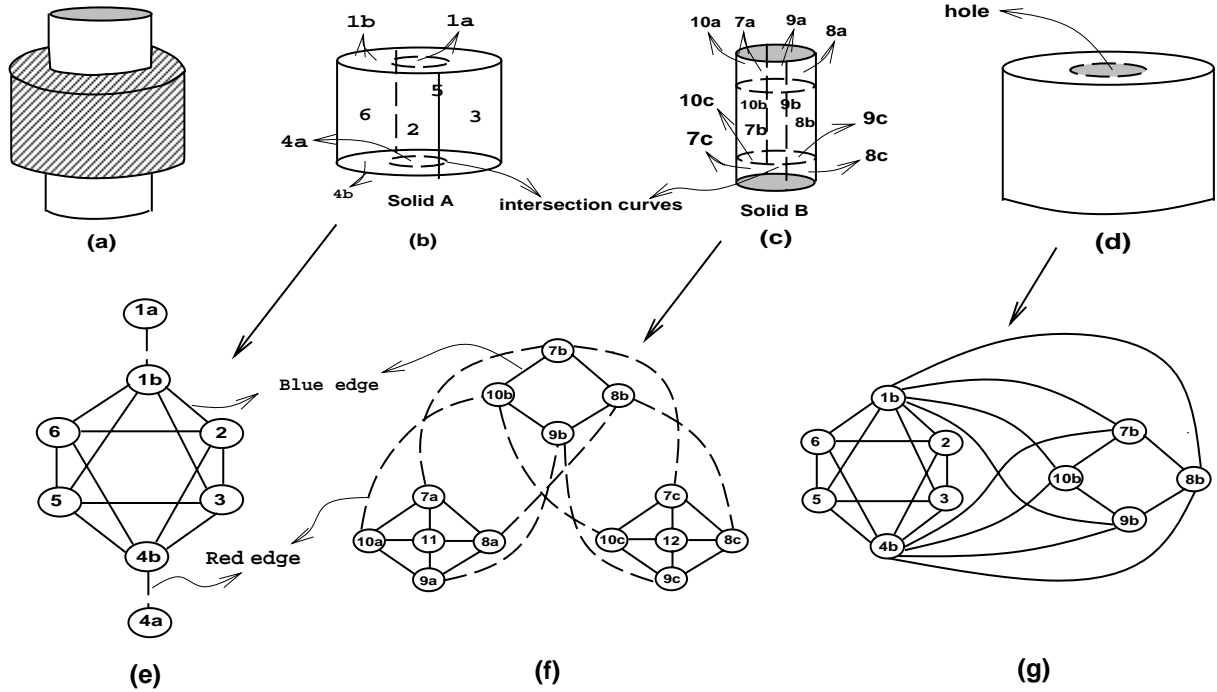
Figure 2 Adjacency Graph Computation for a Difference Operation
