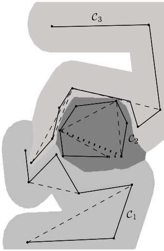
Figure 13: Step 3: Set of compliant proximate shortcut segments (dashed) and compliant nonproximate segments (bold dotted).
