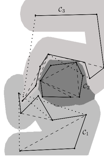
Figure 12: Step 2: Set of compliant shortcut segments (dashed) and non-compliant shortcut segments (bold dotted)
