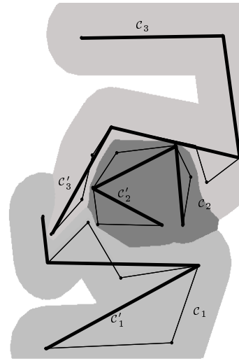
Figure 14: Step 4: Simplified chains (bold) and Input chains.
