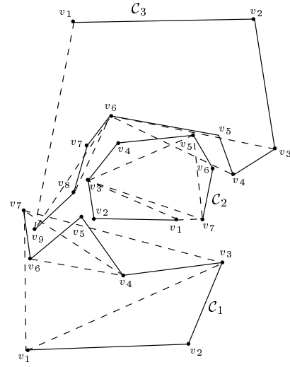
Figure 9: Preprocessing: Input chains (solid) together with the initial set \mathcal{S} of candidate segments (dashed).
