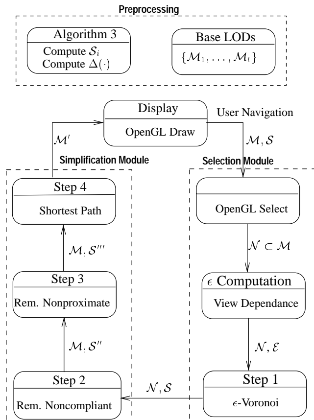
Figure 15: System components of our Map viewer
