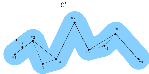
Figure 3: A simplified chain \mathcal{C}' = \{v_1, v_2, v_4, v_5, v_6, v_8, v_9\} (solid line) of input chain \mathcal{C} (dotted line), with \text{size}(\mathcal{C}') = 7 , and d(\mathcal{C}', \mathcal{C}) \leq \epsilon .
