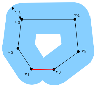
Figure 6: An example of a non-proximate segment \overline{v_1v_6} (in red) completely inside the region defined by the Minkowski sum.
