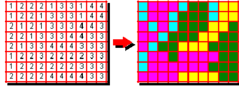
Figure 10: Stencil region with corresponding color buffer.
