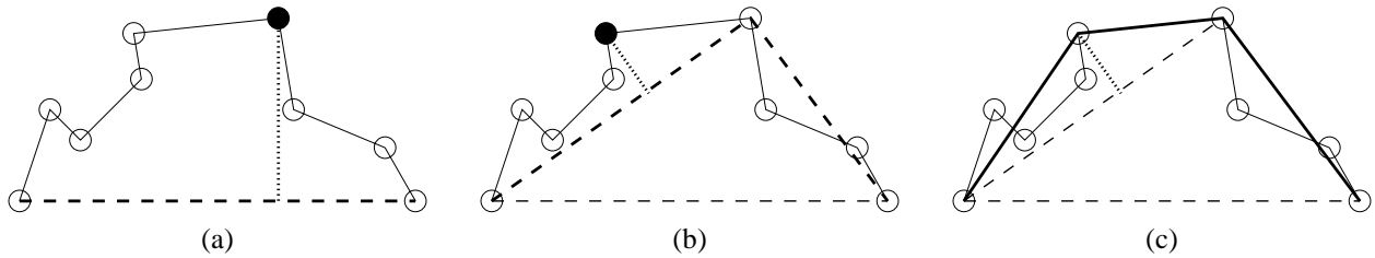
Figure 4: An illustration of the Douglas-Peucker algorithm.
