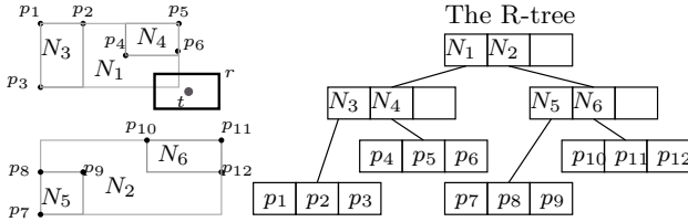
Fig. 2. The R-tree.
