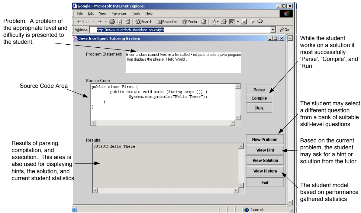
Figure 4. JITS User Interface
