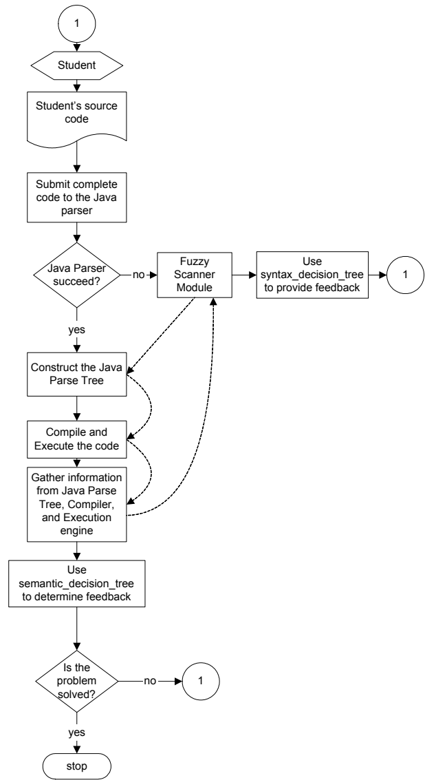
Figure 2. Flowchart of JITS AI Module
