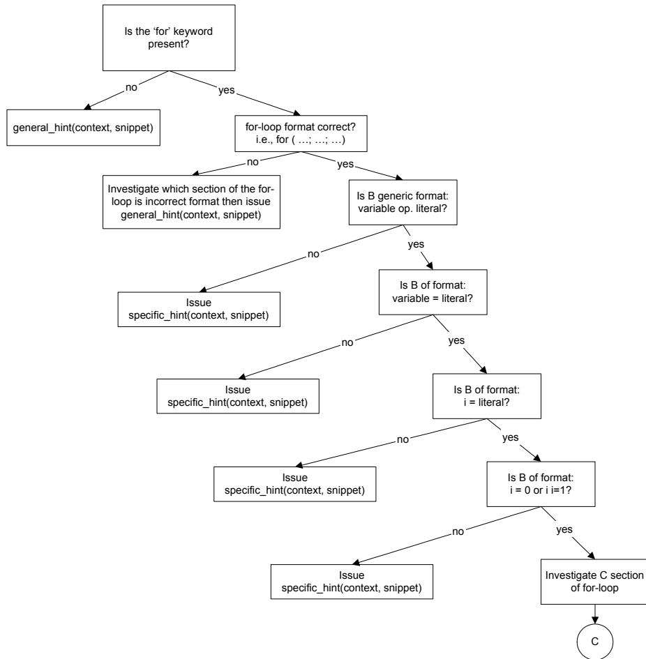
Figure 3. JITS semantic_decision_tree (sections A and B from Figure 1 only)
