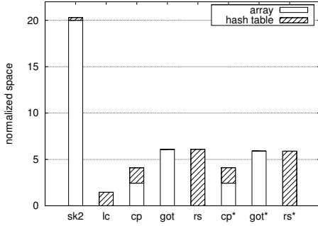
(b) trace = ISP-100k, gran = 8, \epsilon = 0.001
