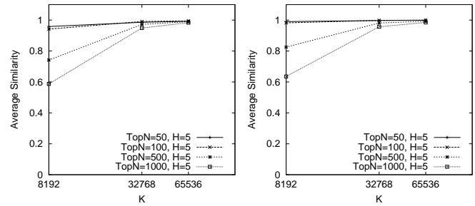
(a) Router=large
