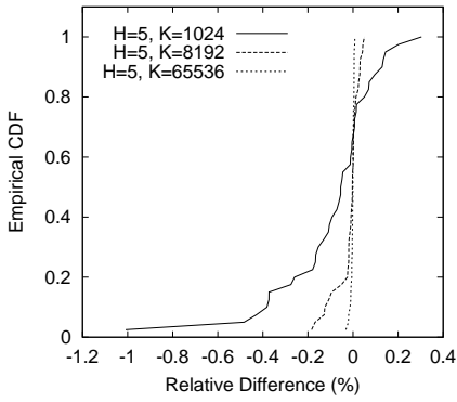
(b) Model=ARIMA0
