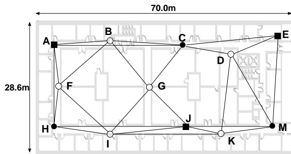
Figure 9: Experiment layout. In our backbone experiment, 50% of the nodes (B, D, F, G, I, K) are in sleep mode. Nodes with square (A, E, J) are leaders, nodes in black dots (C, H, M) are bridges.
