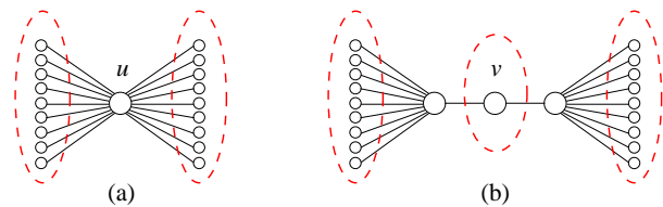
Figure 2: Dashed ovals represent likely volunteers. (a) A large one-hop neighborhood reduces u ’s probability of volunteering, whereas (b) a large two-hop neighborhood has the opposite effect.
