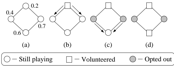
Figure 1: An example GVTD game run on (a) a sample graph. (b) The top-most node volunteers and notifies its neighbors who (c) opt out and inform their neighbor, who then (d) volunteers immediately.
