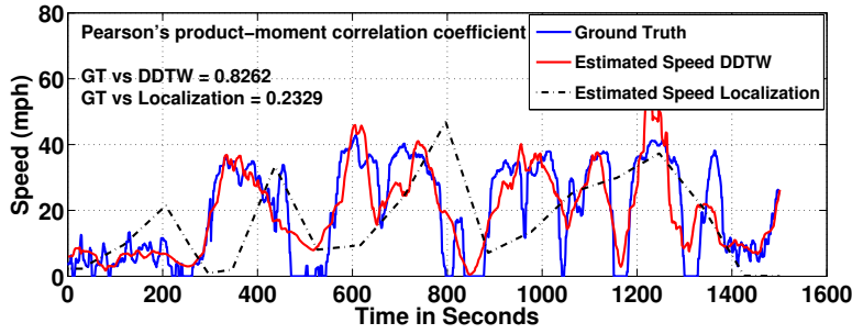
(a) Ground truth and estimated speeds of DDTW and Localization
