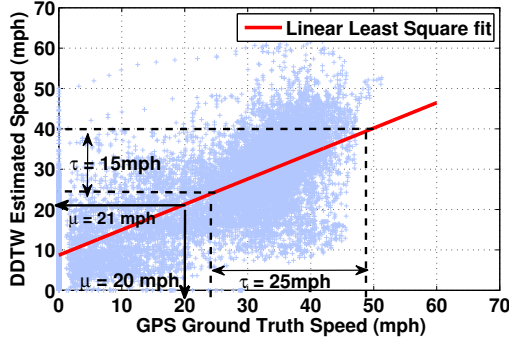
Fig. 4. Least square fit between the ground-truth speed from GPS and the estimated speed from DDTW.
