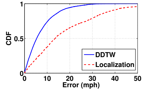
(b) CDF of the speed estimation error
