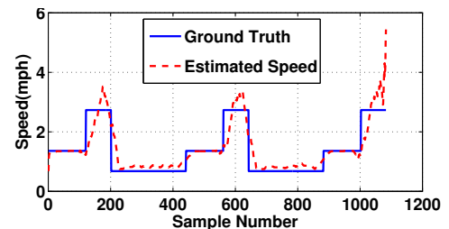
Fig. 9. Speed estimates from DDTW on indoor environment using RSS from receiver-1
